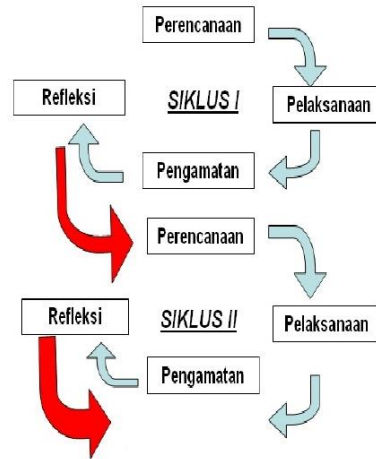
Gambar 1 Prosedur Penelitian
