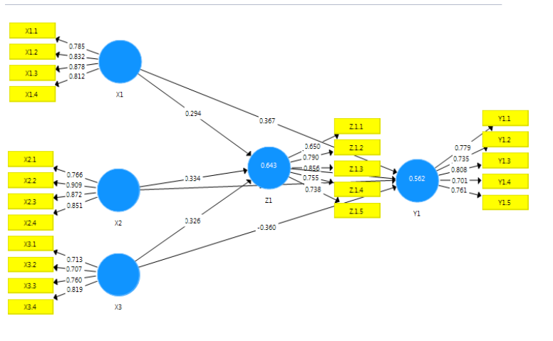
Gambar 1. Pengujian Outer Model
